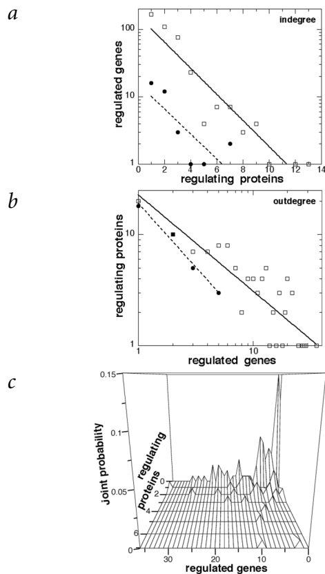
Fig. 2 Connectivity of the yeast genetic network. a , Arriving connectivity distribution (semi-log plot). The number of regulating proteins per regulated gene follows an exponential distribution (least-square method) both for all 402 regulated genes (367 nonregulatory and 35 interregulatory genes—17 interregulatory genes are excluded because they lack a known regulator; 909 connections; open squares, full line; p_k=157e^{-0.45k} ; R=0.99 ) and for the subset of 35 interregulatory genes (72 connections; filled circles, broken line; p_k=15e^{-0.43k} ; R=0.94 ). b , Departing connectivity distribution (log/log plot). The number of regulated genes per regulating protein better fits a power-law distribution both for all 124 regulating proteins (909 connections; open squares, full line; P_k=23k^{-0.87} ; R=0.95 ) and for its subset of 37 regulating proteins that control regulatory genes (72 connections; filled circles, broken line; P_k=19k^{-1.14} ; R=0.99 ). Opposite views (a versus b; exponential departing and power-law arriving connectivities) would give lower correlation coefficients ( R=0.88, 0.91, 0.83 and 0.98 , respectively) and very different slopes for global versus interregulatory genes. Null values were discarded. c , Joint distributions. The probability that a randomly chosen gene has in arriving and out departing connections is distributed on this linear plot as a function of in (regulating proteins) and out (regulated genes).
